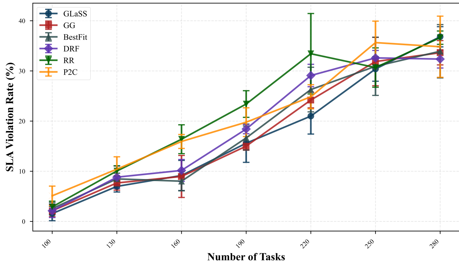
SLA Violation Rate vs Task Count (Bursty Mode)
